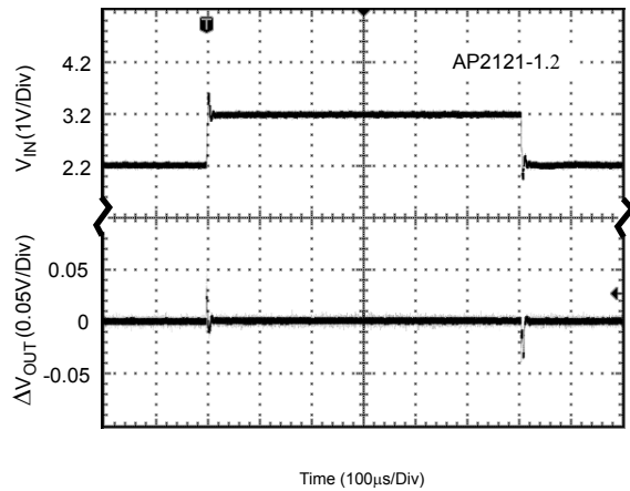
Figure 19. Line Transient (Conditions: I OUT =30mA, C IN =1μF, C OUT =1μF)
